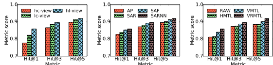
(a) Effect of multi-view graphs. (b) Effect of route representation learning. (c) Effect of hierarchical multi-task learning.
