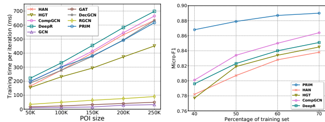
Figure 5: Training scalability Figure 6: Results on sparse cases
