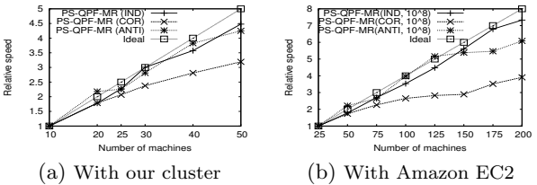
Figure 9: Relative speedups with |\mathbb{D}| = 10^8
