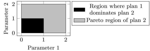
Figure 5: Pareto regions are not necessarily convex.
