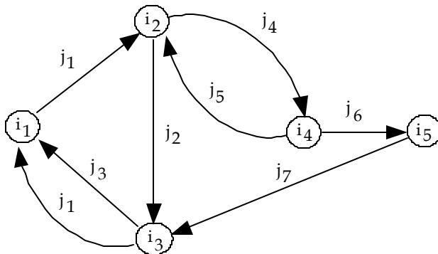
Figure 2: Network G'
