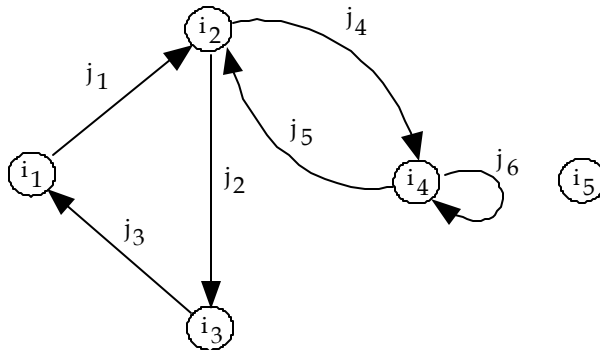
Figure 1: Network G
