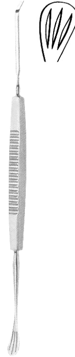
PATON DOUBLE ENDED SPATULA With groove, 6.0mm x 15.0mm and 2.0mm x 31.0mm, end of blade angled up 7.0mm 601-105 5 3 / 4 "
