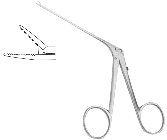
HOUSE Forceps
