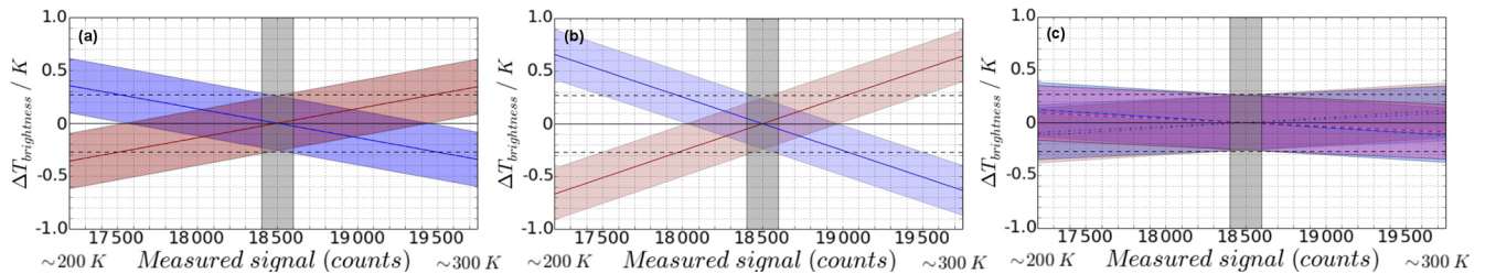
Figure 12. Error estimation of calibration methods with the applied HALO TS (assumed to be at 250 K) offset correction for the calibration methods (a) noise diode + hot target, (b) hot target + HALO TS, and (c) using cold-chamber calibration parameters. The measurement error for an individual measurement is indicated by the uppermost and lowermost edges of the blue or red shaded region (caused by measurement noise). Vertical grey shaded region: expected range of measurement signals if the 0^\circ measurement signal is at 18 500 counts ( \approx 250 K). Black dashed horizontal lines: expected error induced by measurement noise of 6 counts.
