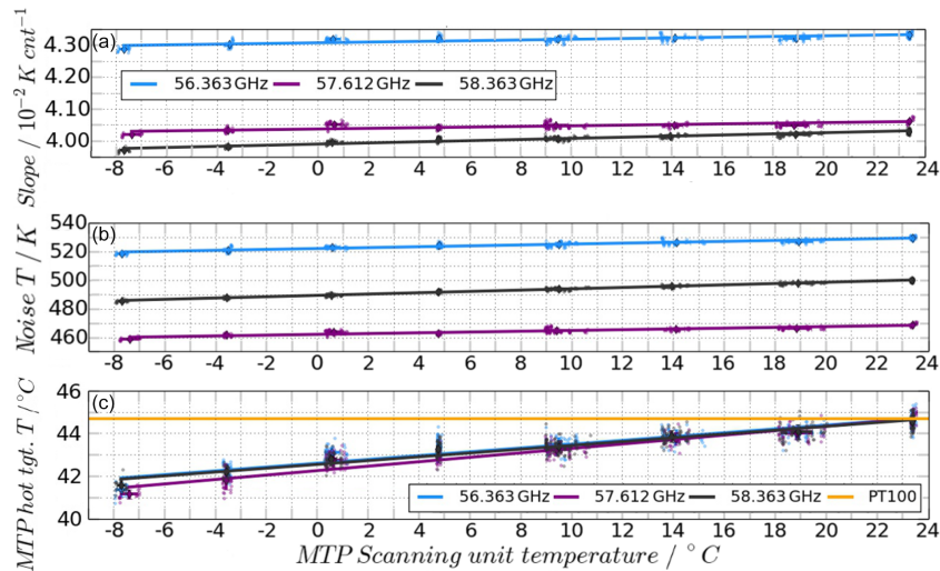
Figure 8. Calibration parameters calculated from hot–cold calibration for standard frequency channels during cold-chamber measurements. (a) Slope of calibration line. (b) Receiver noise temperature ( T_R ). (c) Calculated hot target TBs at different scanning unit temperatures during cold-chamber measurements. Small dots: single measurements contributing to the average at one scanning unit temperature. Orange line: Pt100 sensor readings.
