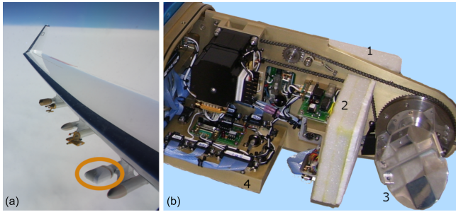
Figure 1. HALO MTP instrument. (a) Position of the MTP underneath the wing of the HALO aircraft. (b) MTP sensor unit in the lab. Marked with numbers are the radiometer unit (1), the hot calibration target (2), the rotating mirror (3), and the electronic unit (4), which contains various temperature sensors such as the scanning unit temperature and the pod air temperature sensor.
