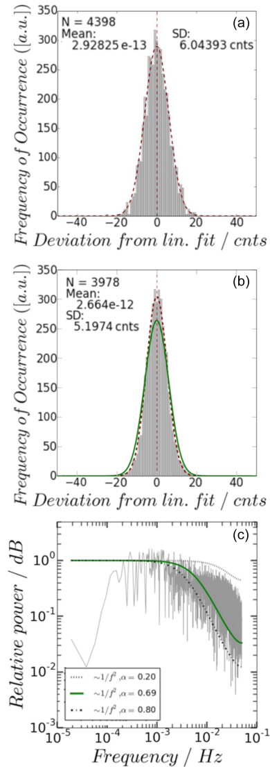
Figure 7. HALO MTP noise characteristics at 56.363 GHz. Figures for the other two standard frequency channels look similar. Fit parameters for all three frequency channels are summarized in Table 2. (a) Laboratory measurements in the cold chamber. Red dashed line: Gauss fit to the data. (b) Derived from ML CIRRUS flight data. Green line: ideal Gauss function with the mean at 0.0 and a standard deviation of 6 counts ( \sim 0.25 K), as implied by the cold-chamber noise spectrum. (c) Noise spectrum calculated from ML CIRRUS flight data. Black dashed lines: theoretical power spectra of 1/f^2 noise with lag-1 correlations of \alpha = 0.2 and \alpha = 0.8 . Green solid line: theoretical power spectrum of 1/f^2 noise with lag-1 correlation of input data.
