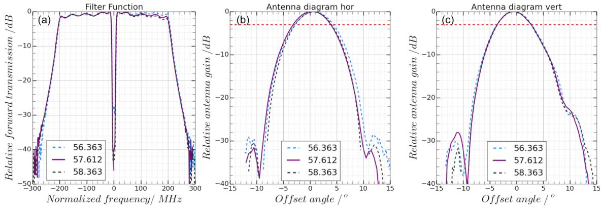
Figure 2. HALO MTP filter functions (a) and antenna diagram of the horizontal (b) and vertical (c) plane recorded at standard measurement frequencies. Red dashed lines indicate the half-maximum value. All data are normalized so that the maximum value shown is 0.
