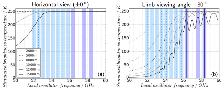
Figure A2. Simulated TBs at frequency channels between 50 and 60 GHz at different flight altitudes (different line styles) for a horizontal viewing angle (a) and a near-zenith angle (b). Solid vertical lines: standard frequency channels of the MTP; dashed vertical lines: strong lines that could be used as new MTP LOs. Shading around vertical lines: MTP filter width. Lines corresponding to altitudes of 8 km or lower overlap in panel (a).
