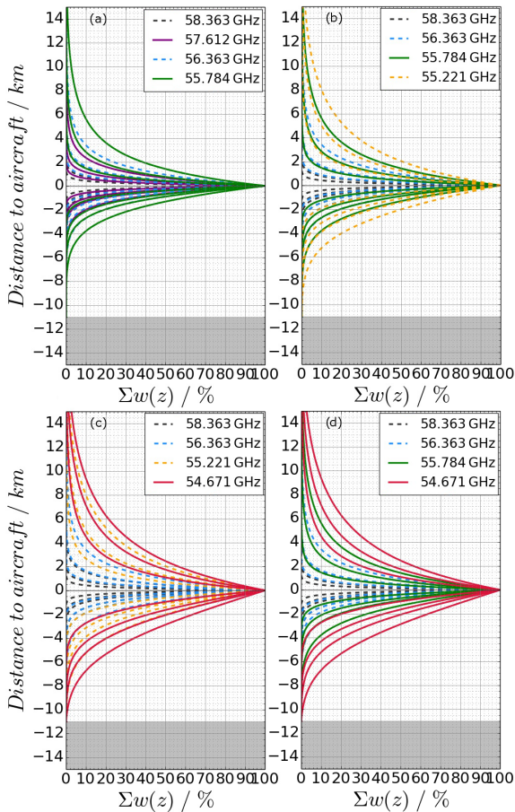
Figure A3. Cumulated weights of the MTP frequency channels (with each individual line in a panel corresponding to a different viewing angle and frequency combination) calculated for an aircraft altitude of 11 km. Shown are possible new measurement strategies, as mentioned in Table A2: (a) 8E4LOa, (b) 8E4LOc, (c) 8E4LOb1, and (d) 8E4LOb2. Grey areas at the bottom: altitude range that would be below the surface.
