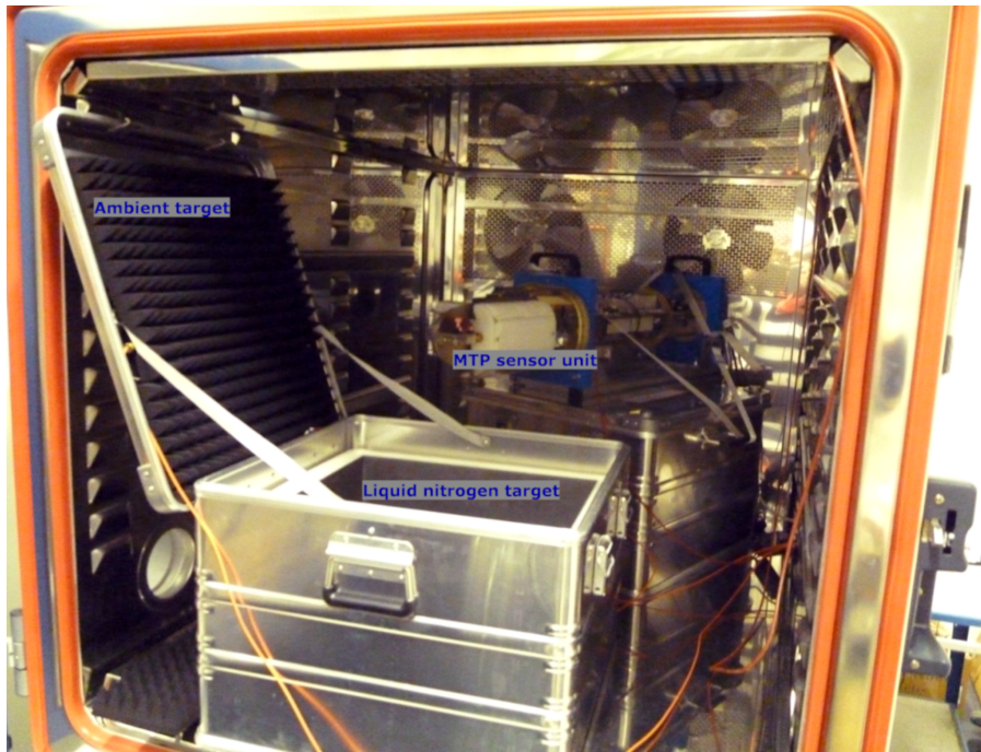
Figure 3. HALO MTP inside the cold chamber. For the measurements, the box containing the liquid nitrogen and the ambient target was rotated to face towards the MTP sensor unit. A second microwave absorber was placed on the ceiling of the chamber to function as a second ambient target.
