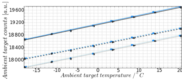
Figure 5. Ambient target temperature vs. the measured signal (counts) of the two ambient targets for all three standard frequency channels of the HALO MTP (different line styles). Different line colors correspond to the measurement of the two individual ambient targets.
