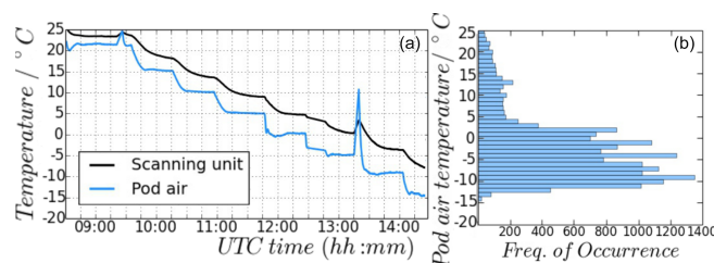
Figure 4. Temperature sensor measurements during cold-chamber measurements (a; black line: scanning unit sensor, blue line: pod air sensor). At 0^\circ\text{C} ( \sim 11:45 UTC) the cold-chamber software had to be restarted, causing a longer stabilization period, and at -5^\circ\text{C} ( \sim 13:15 UTC) the cold chamber was opened to refill the liquid nitrogen in the cold target, causing spikes in the temperature measurement. (b) Pod air temperature measurements during all ML CIRRUS campaign flights.
