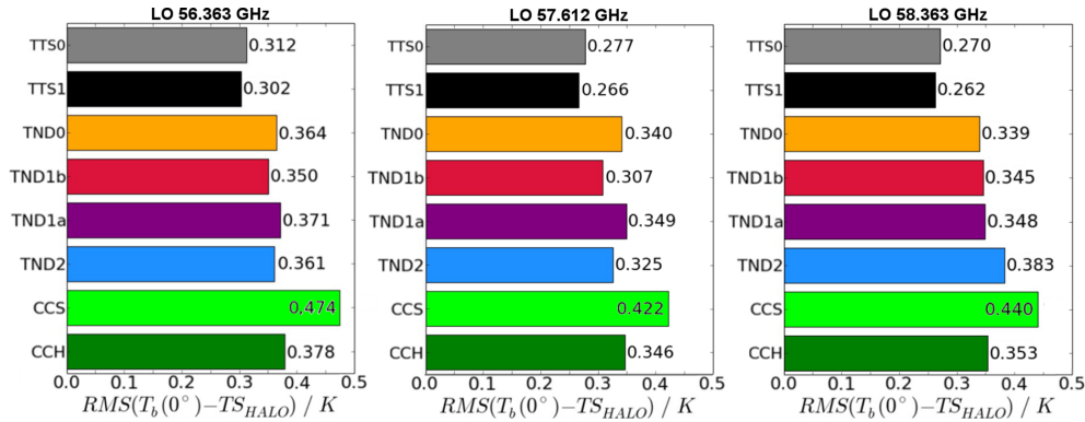
Figure 11. The rms difference between HALO TS and TBs derived from the MTP measurement signal at a limb-viewing angle of 0° at the three standard frequency channels during all ML CIRRUS flight segments with no altitude changes, curves, or ND failures with signals longer than 10 min. Refer to Table 6 for the denominations of the calibration methods.
