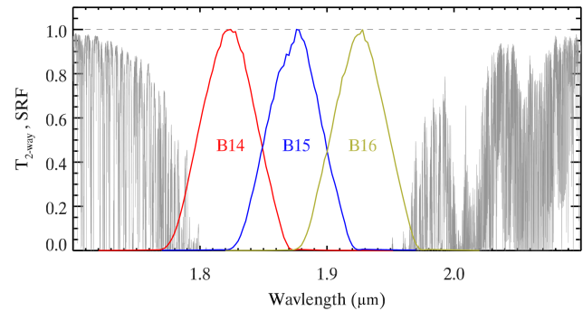
Figure 1. Spectral two-way transmittance (gray line), from TOA to surface, calculated with LBLRTM using a tropical ocean atmosphere. Spectral response functions during the SEAC 4 RS campaign for eMAS bands 14, 15, and 16 (band centers at approximately 1.83, 1.88, and 1.93 \mu\text{m} , respectively) are also shown (red, blue, and gold lines, respectively).
