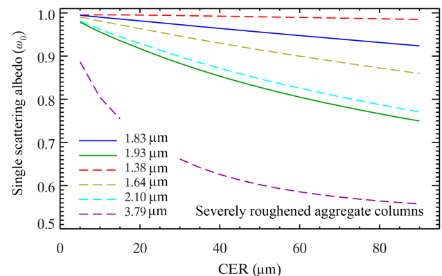
Figure 2. Bulk single scattering albedo ( \omega_0 ) for severely roughened aggregate hexagonal column ice crystals as a function of cloud effective particle radius (CER) for the eMAS 1.83 and 1.93 \mu\text{m} channels (blue and green, respectively) and the MODIS 1.38, 1.64, 2.1, and 3.79 \mu\text{m} channels (dotted red, gold, light blue, and magenta, respectively).
