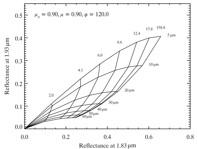
Figure 3. Two-channel plot illustrating the sensitivity of the 1.83 and 1.93 \mu\text{m} eMAS channels to cloud optical thickness (near-vertical lines) and effective particle radius (near-horizontal lines), respectively.
