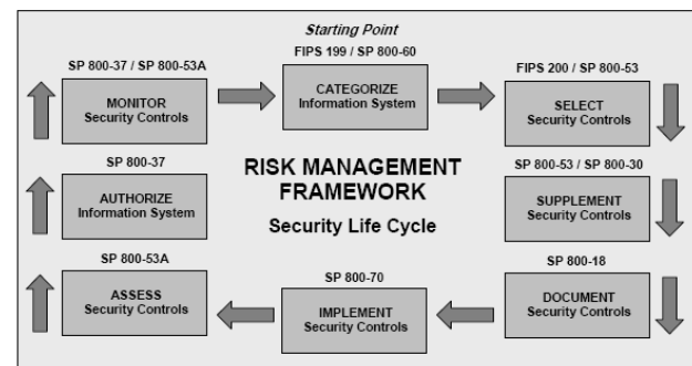
Fig. 1. Risk Management Framework (From [3])
