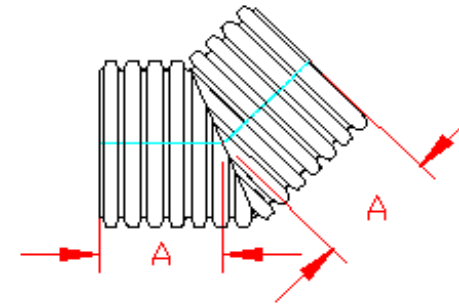
PLAIN END
