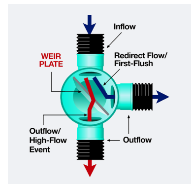
Weir Structure
