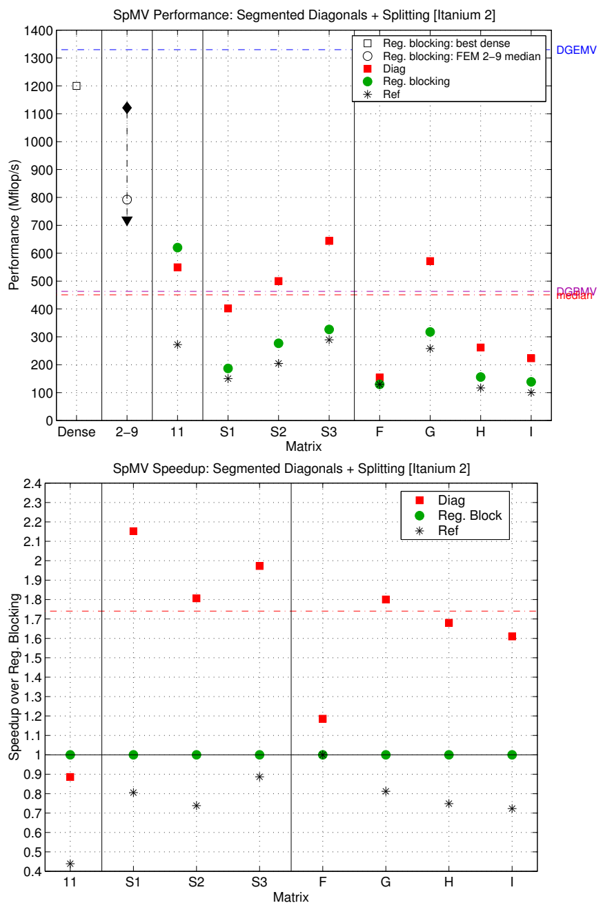
Figure 5.18: Performance results on diagonal matrices: Itanium 2. (Top) Performance in Mflop/s (Bottom) Speedup of the RSDIAG implementation over register blocking. This data is also tabulated in Table H.4.
