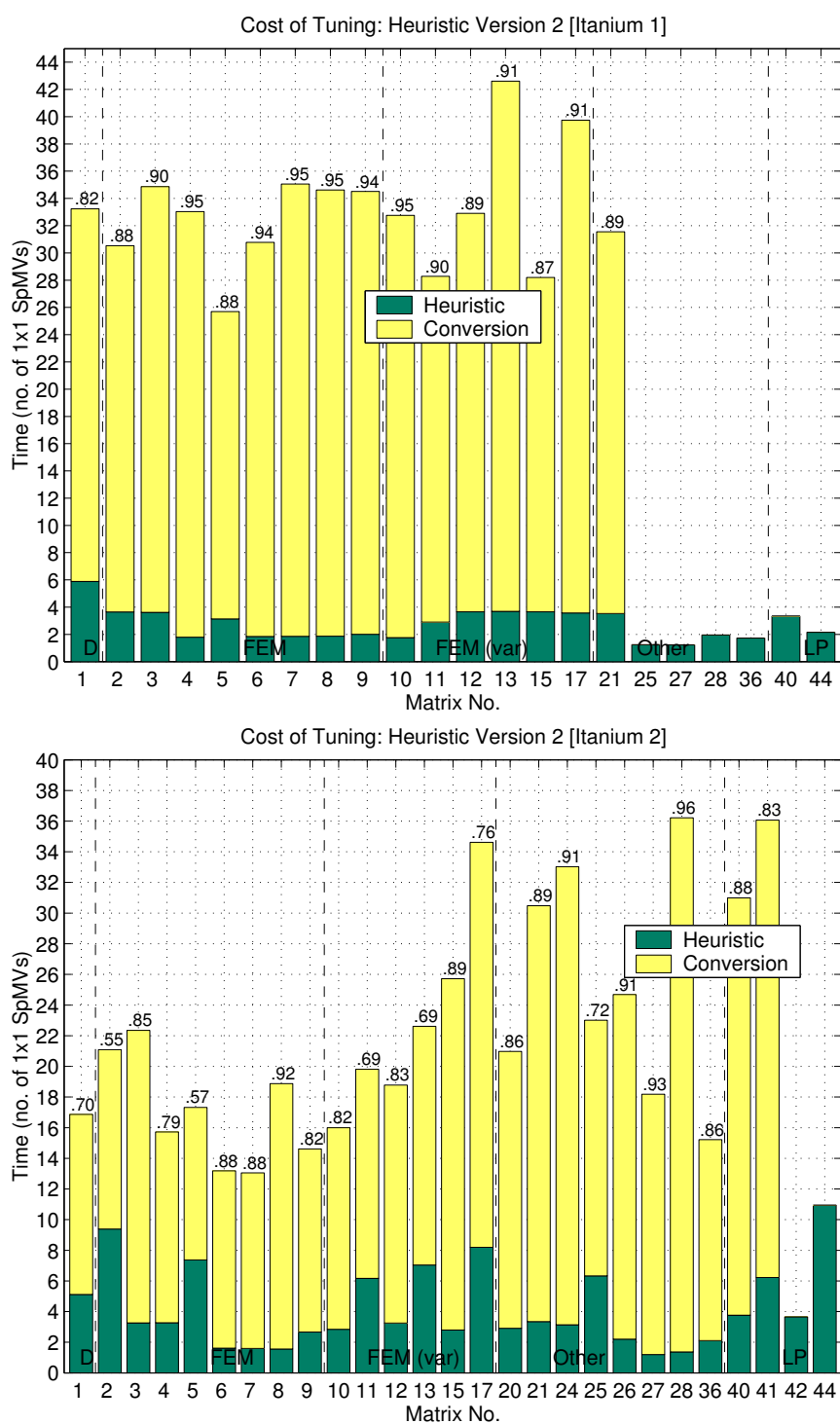
Figure 3.19: Cost of register block size tuning: Itanium 1 and Itanium 2. (Top) Itanium 1 (Bottom) Itanium 2
