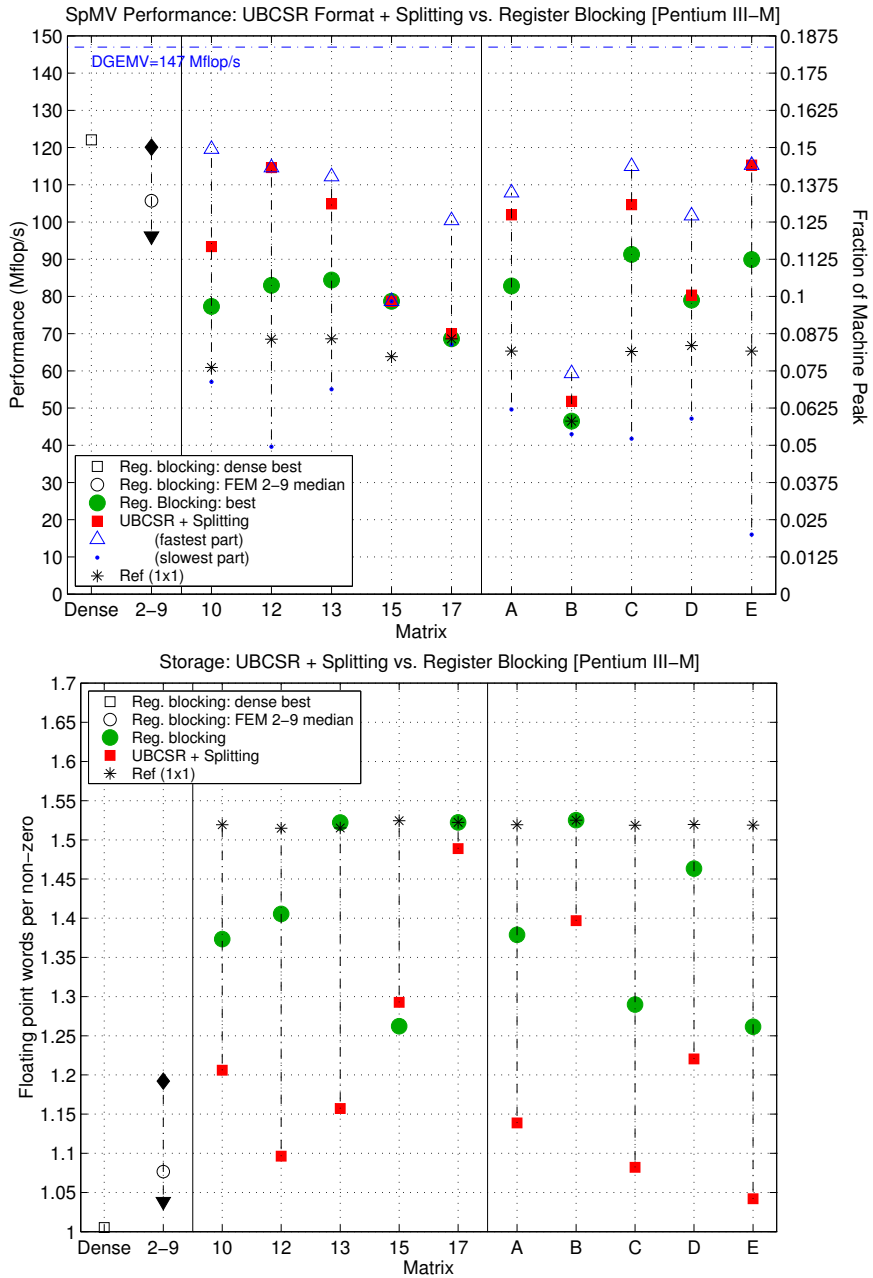
Figure 5.7: Performance and storage for variable block matrices: Pentium III-M. (Top) Performance, Mflop/s. (Bottom) Storage, in doubles per ideal non-zero. For additional data on the block sizes used, see Table G.2.
