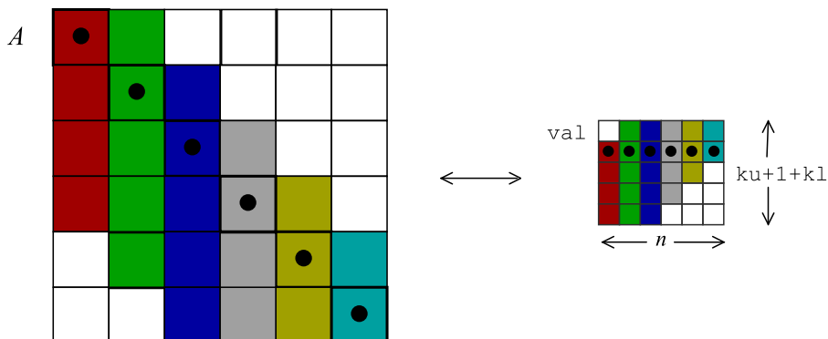
Figure 2.5: Dense band format. Here, a banded matrix A in dense band (column-major) format is stored in a (\mathbf{ku} + 1 + \mathbf{k1}) \times n array val , where \mathbf{ku} is the upper-bandwidth and \mathbf{k1} is the lower-bandwidth. In this example, \mathbf{ku} = 1 and \mathbf{k1} = 3 , and columns are stored contiguously in val . The main diagonal has been marked with solid black dots to show that diagonal elements lie in a row of val .
