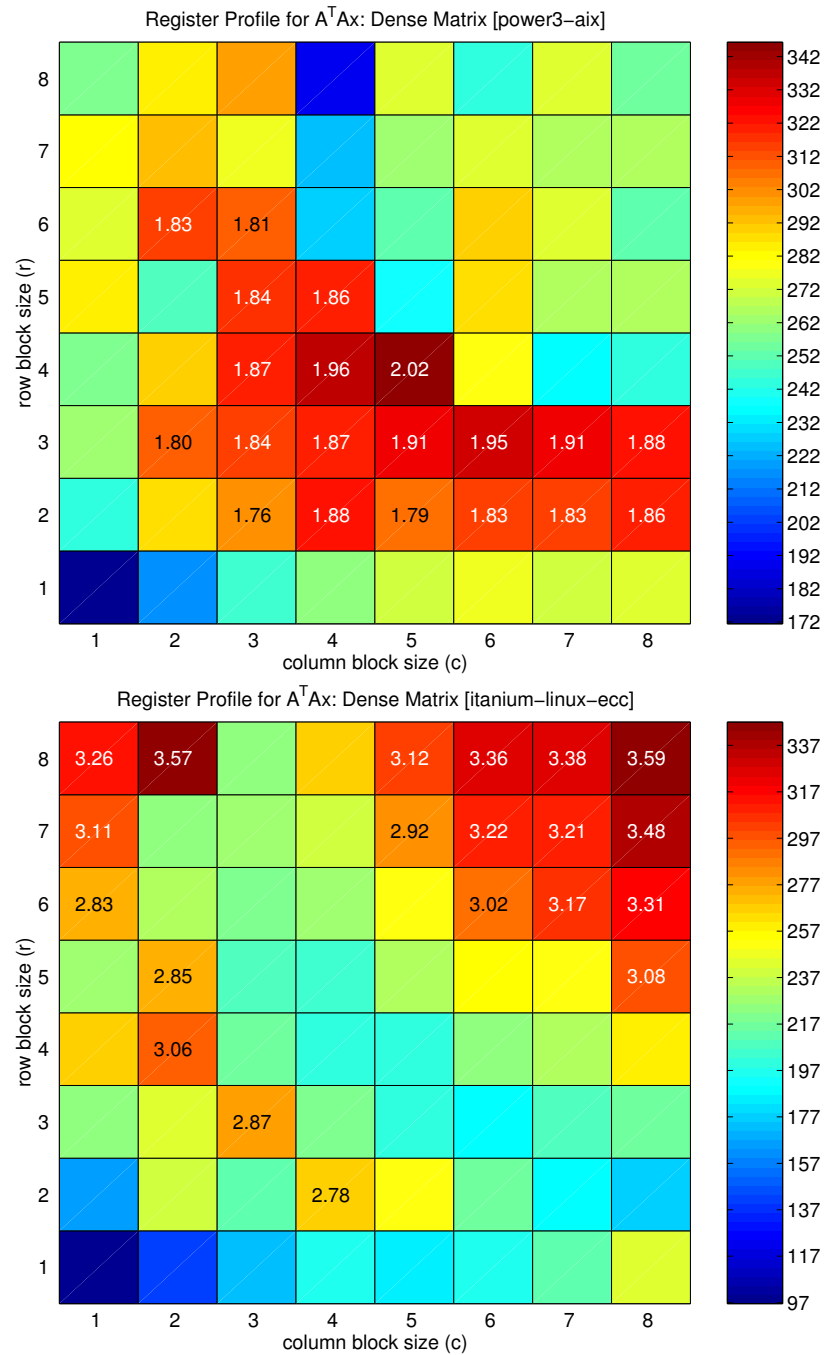
Figure 7.3: Cache-optimized, register blocked A^T A \cdot x performance profiles (offline benchmarks) capture machine-dependent structure: Power3 and Itanium 1. We show the performance of the cache-optimized, register blocked code on a dense matrix stored in sparse r \times c format, for all r \times c up to 8 \times 8 . Each square is an implementation, shaded by its performance (Mflop/s) and labeled by its speedup over the unblocked ( 1 \times 1 ), cache-optimized code. ( Top ) Profile for the Power3. ( Bottom ) Itanium 1.
