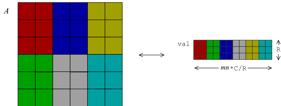
Figure 2.3: Dense block-major format. In block-major format, R \times C submatrices are stored contiguously in blocks in val . Each block may furthermore be stored in any dense matrix format (e.g., column major, row major, ...). Here, A is 6 \times 6 and R = 3 , C = 2 .
