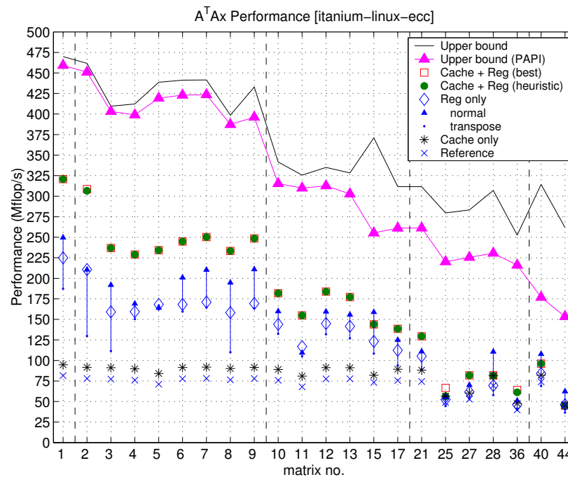
Figure 7.9: A^T A \cdot x performance on the Intel Itanium platform. A speedup version of this plot appears in Appendix I.3.
