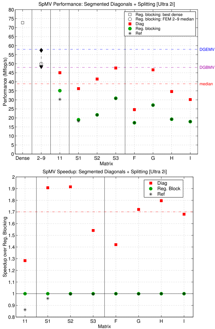
Figure 5.15: Performance results on diagonal matrices: Ultra 2i. (Top) Performance in Mflop/s of (Bottom) Speedup of the RSDIAG implementation over register blocking. This data is also tabulated in Table H.1.
