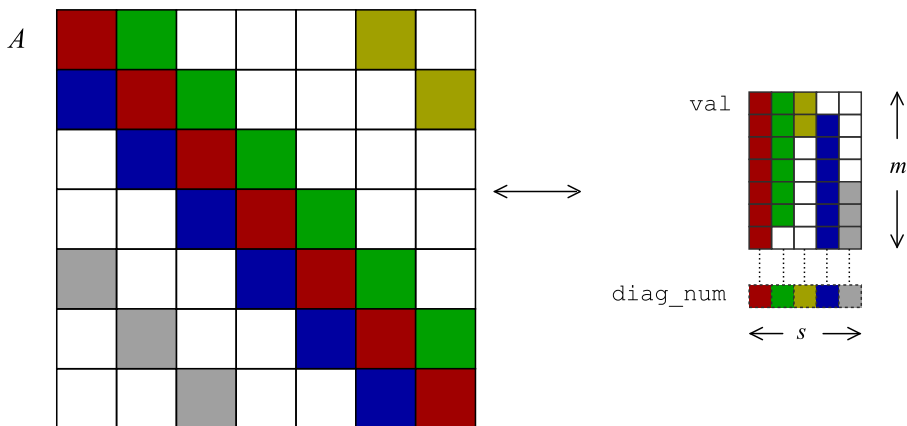
Figure 2.9: Diagonal format (DIAG) . Elements of each diagonal of A are stored continuously in a column of \text{val} . Upper-diagonals are stored beginning in the first row of \text{val} , and lower-diagonals are stored ending at in the last row of \text{val} . Each element \text{diag\_num}[l] of \text{diag\_num} indicates which diagonal is stored in column l of \text{val} .
