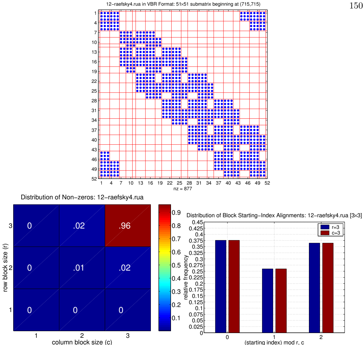
Figure 5.3: Logical grid (block partitioning) after greedy conversion to variable block row (VBR) format: Matrix 12-raefsky4. (Top) We show the logical block partitioning after conversion to VBR format using a greedy algorithm. (Bottom-left) Approximately 96% of the non-zero blocks are 3x3. (Bottom-right) Let (i, j) be the starting row and column index of each 3x3 block. We see that 37.5% of these blocks have i mod 3 = 0, 26% have i mod 3 = 1, and the remaining 36.5% have i mod 3 = 2. The starting column indices follow the same distribution, since the matrix is structurally (though not numerically) symmetric.
