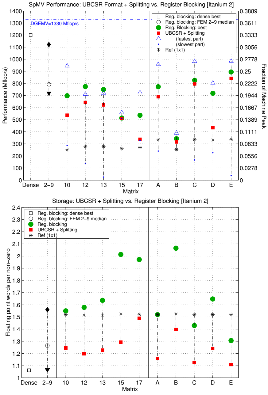
Figure 5.9: Performance and storage for variable block matrices: Itanium 2. (Top) Performance, Mflop/s. (Bottom) Storage, in doubles per ideal non-zero. For additional data on the block sizes used, see Table G.4.
