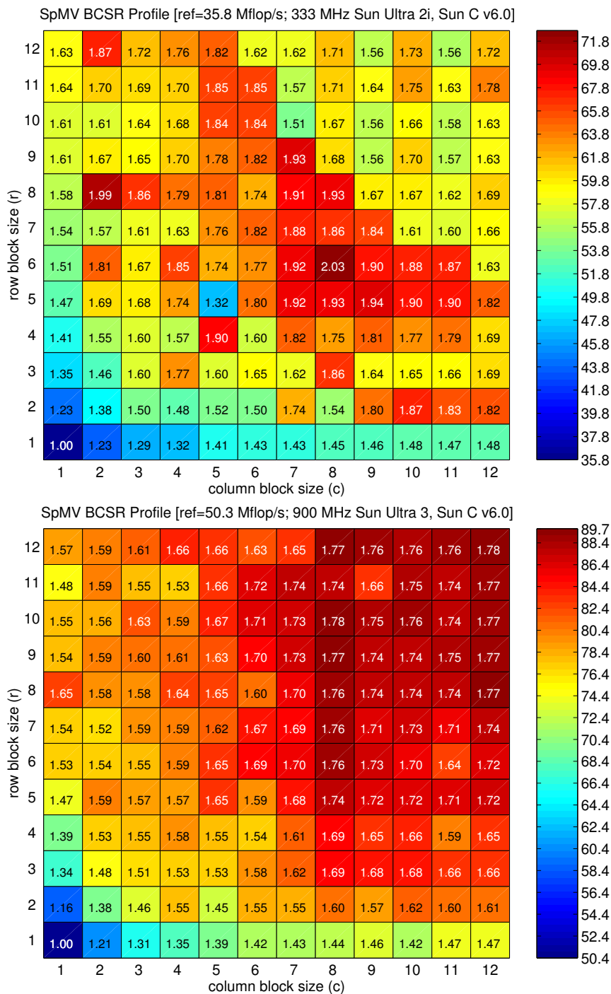
Figure 3.3: SpMV BCSR Performance Profiles: Sun Platforms. The performance (Mflop/s) of r \times c register blocked implementations on a dense n \times n matrix stored in BCSR format, on block sizes up to 12 \times 12 . Results shown for the Sun Ultra 2i ( top ) and Ultra 3 ( bottom ). On each platform, each square is an r \times c implementation shaded by its performance, in Mflop/s. Each implementation is labeled by its speedup relative to the 1 \times 1 implementation.
