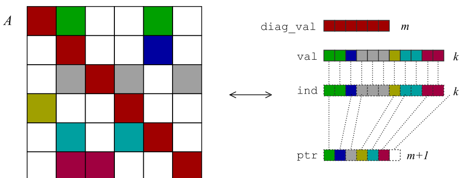
Figure 2.10: Modified sparse row (MSR) format . MSR is identical to CSR, except that the diagonal elements are stored separately in a dense array ( \text{diag\_val} ) where no indexing information need be stored. The off-diagonal elements are stored in CSR format.
