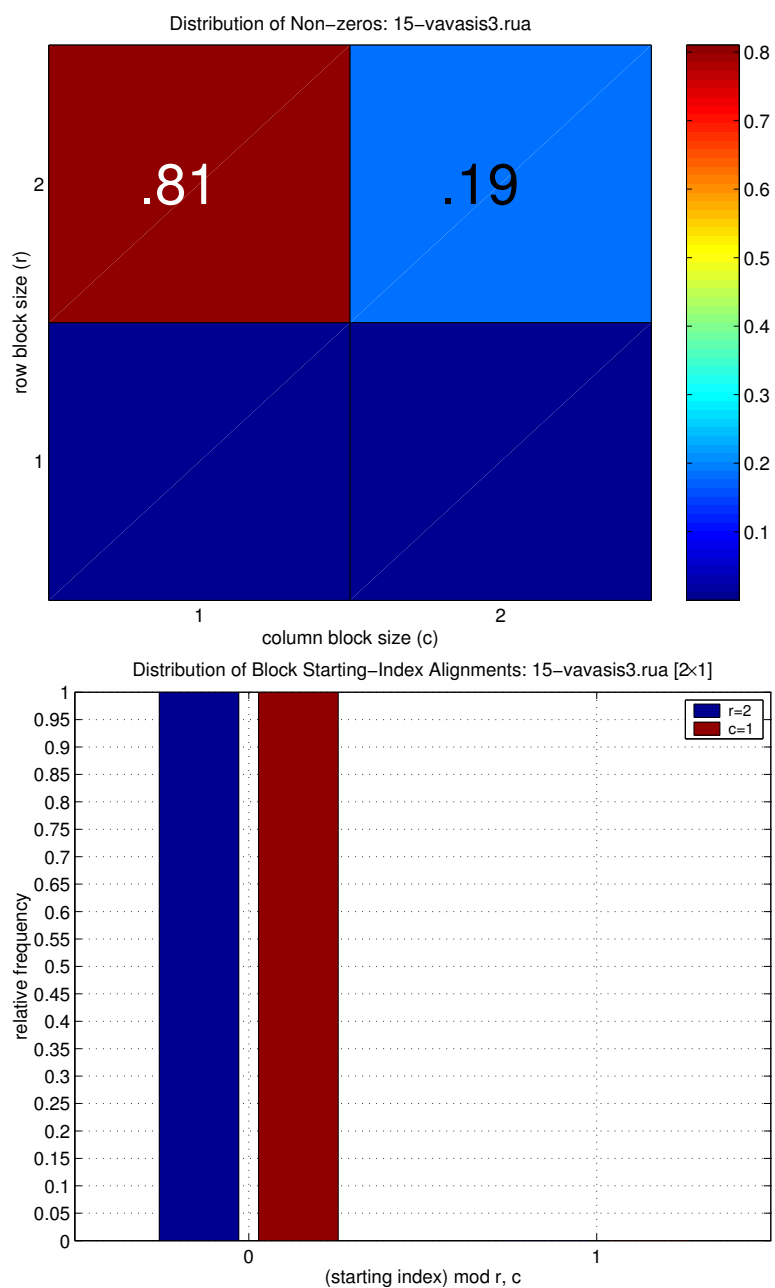
Figure F.14: Distribution and alignment of block sizes: Matrix vavasis3 . ( Top ) Distribution of non-zeros by block size when the matrix is supplied in VBR format with no fill. A numerical label, even if 0, indicates that at least 1 block had the corresponding block size. A lack of a label indicates exactly 0 blocks of the given block size. ( Bottom ) Distribution of row and column alignments for the 2 \times 1 blocks. Specifically, we plot the fraction of 2 \times 1 blocks whose starting row index i satisfies i \bmod r = 0 , and whose starting column index j satisfies j \bmod c = 0 .
