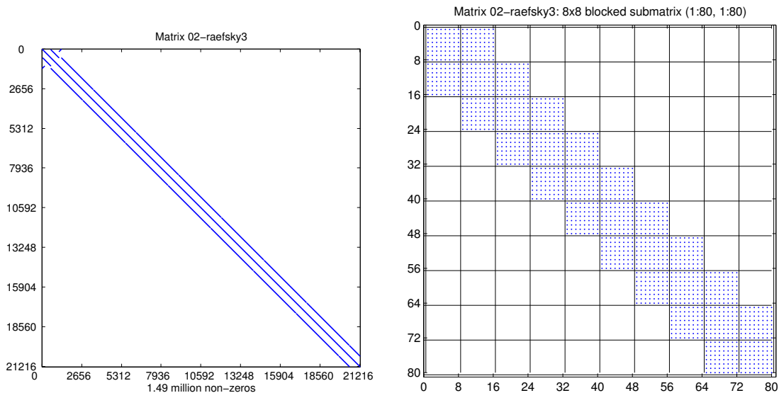
Figure 1.2: Spy plot of sparse matrix raefsky3. (Left) Sparse matrix raefsky3 , arising from a finite element discretization of an object in a fluid flow simulation. This matrix has dimension 21216 and contains approximately 1.5 million non-zeros. (Right) Matrix raefsky3 consists entirely of 8 \times 8 dense blocks, uniformly aligned as shown in this 80 \times 80 submatrix.
