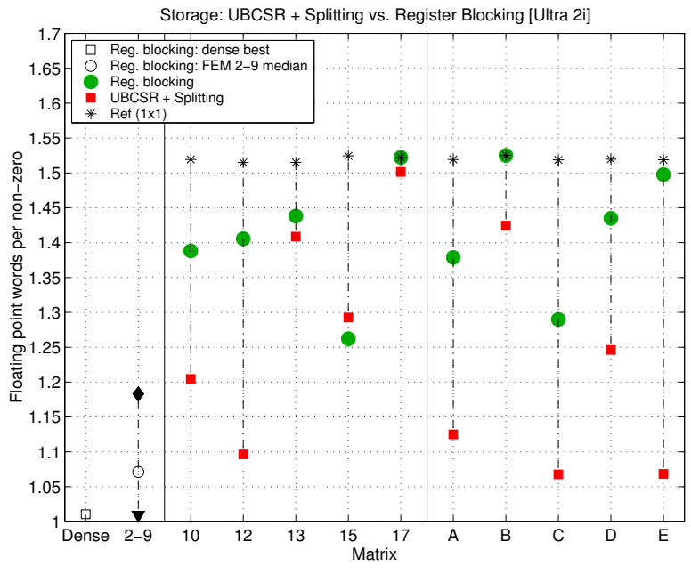
Figure 5.6: Performance and storage for variable block matrices: Ultra 2i. (Top) Performance, Mflop/s. (Bottom) Storage, in doubles per ideal non-zero. For additional data on the block sizes used, see Table G.1.
