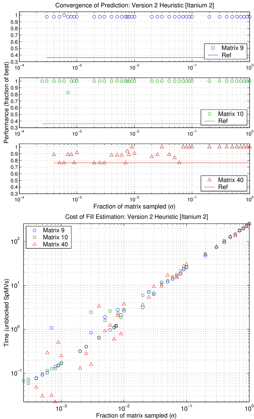
Figure 3.11: Accuracy and cost trade-off example: Matrices 9, 10, and 40 on Itanium 2. (Top) Performance of the implementation chosen by the heuristic as \sigma varies. We show data for three test matrices, where performance (y-axis) is shown as a fraction of the best performance over all 1 \leq r, c \leq 12 . (Bottom) Cost of executing the heuristic as \sigma varies. Time (y-axis) is shown as multiples of the time to execute a single unblocked ( 1 \times 1 ) SpMV on the given matrix. These data are tabulated in Appendix D.
