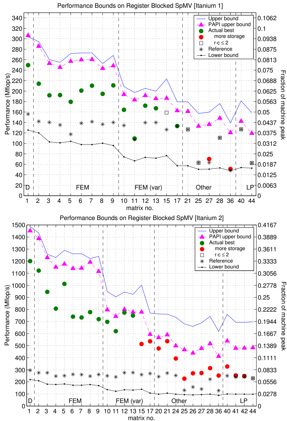
Figure 4.15: Comparison of observed performance to the bounds: Itanium 1 and Itanium 2. ( Top ) Performance data on Itanium 1. DGEMV performance: 315 Mflop/s. Peak: 3.2 Gflop/s. ( Bottom ) Performance data on Itanium 2. DGEMV: 1.33 Gflop/s. Peak: 3.6 Gflop/s.
