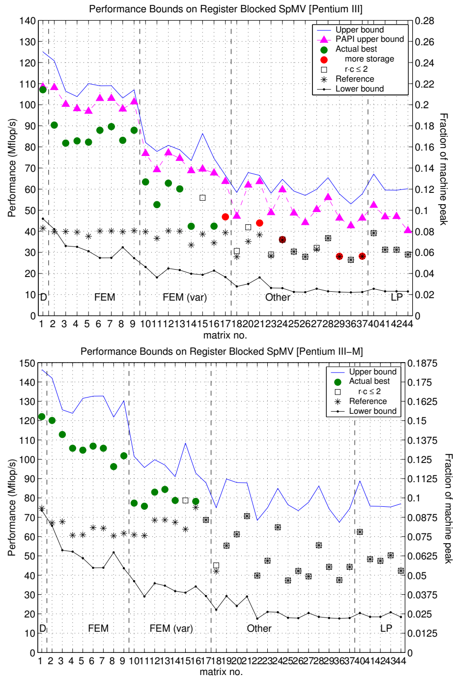
Figure 4.13: Comparison of observed performance to the bounds: Pentium III and Pentium III-M. (Top) Performance data on Pentium III. DGEMV performance: 58 Mflop/s. Peak: 500 Mflop/s. (Bottom) Performance data on Pentium III-M. DGEMV: 150 Mflop/s. Peak: 800 Mflop/s. Note: PAPI was not available on this platform.
