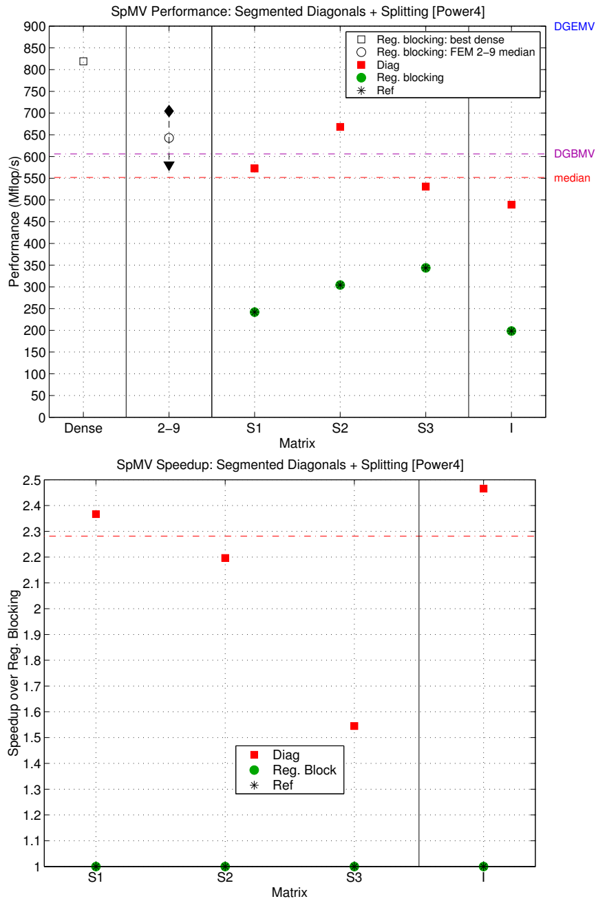
Figure 5.17: Performance results on diagonal matrices: Power4. (Top) Performance in Mflop/s of (Bottom) Speedup of the RSDIAG implementation over register blocking. This data is also tabulated in Table H.3.
