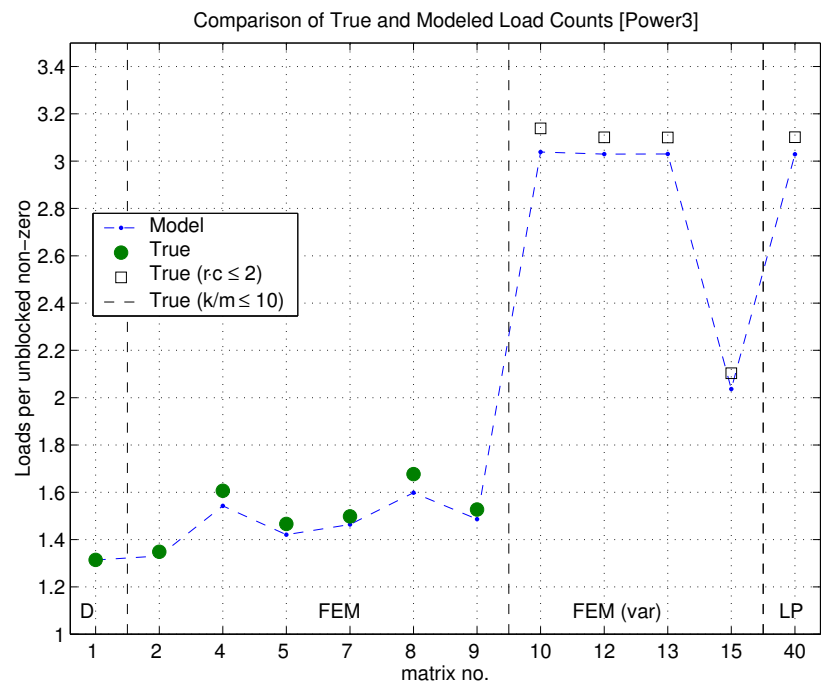
Figure 4.4: Comparison of analytic and measured load counts: Power3.
