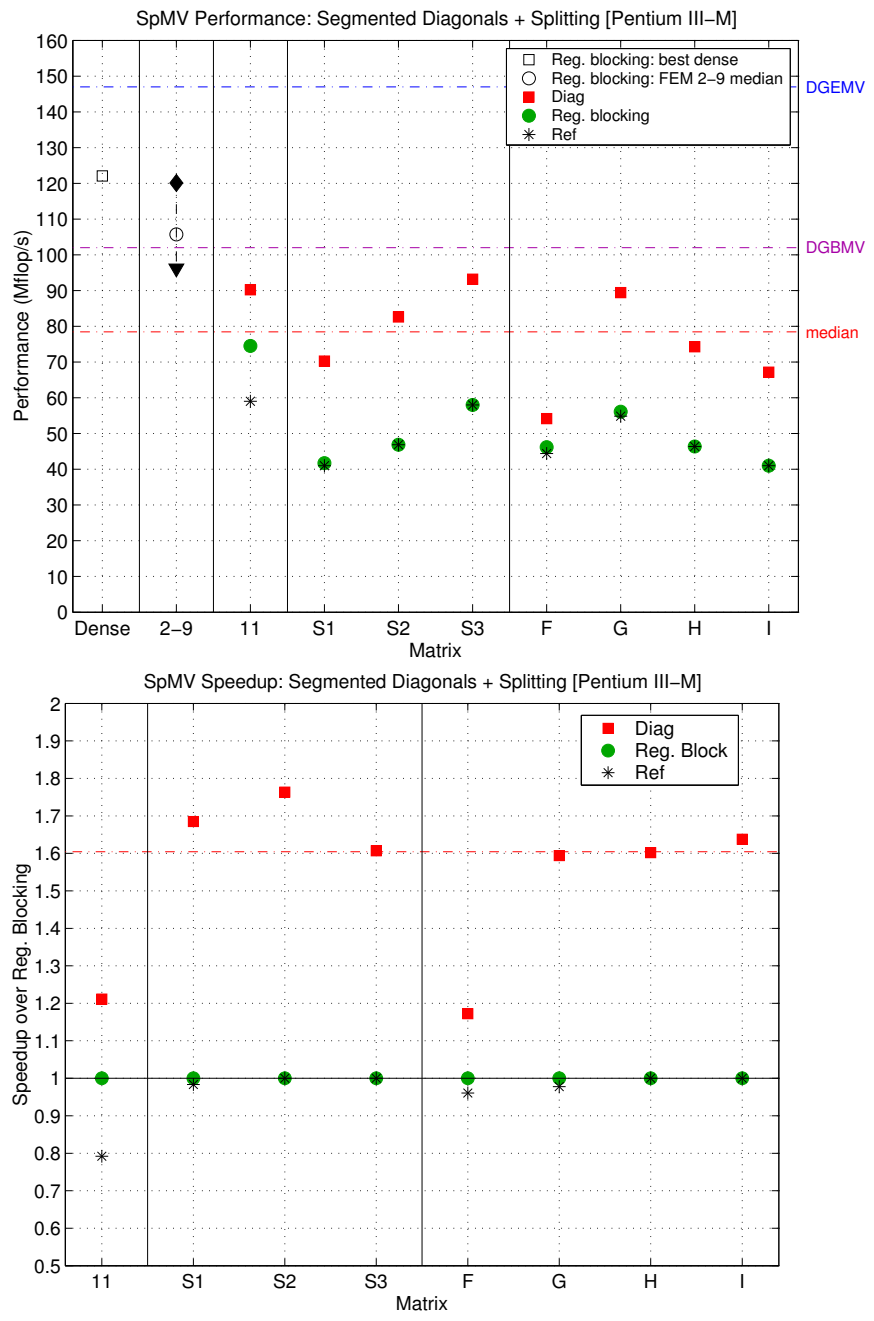
Figure 5.16: Performance results on diagonal matrices: Pentium III-M. (Top) Performance in Mflop/s (Bottom) Speedup of the RSDIAG implementation over register blocking. This data is also tabulated in Table H.2.
