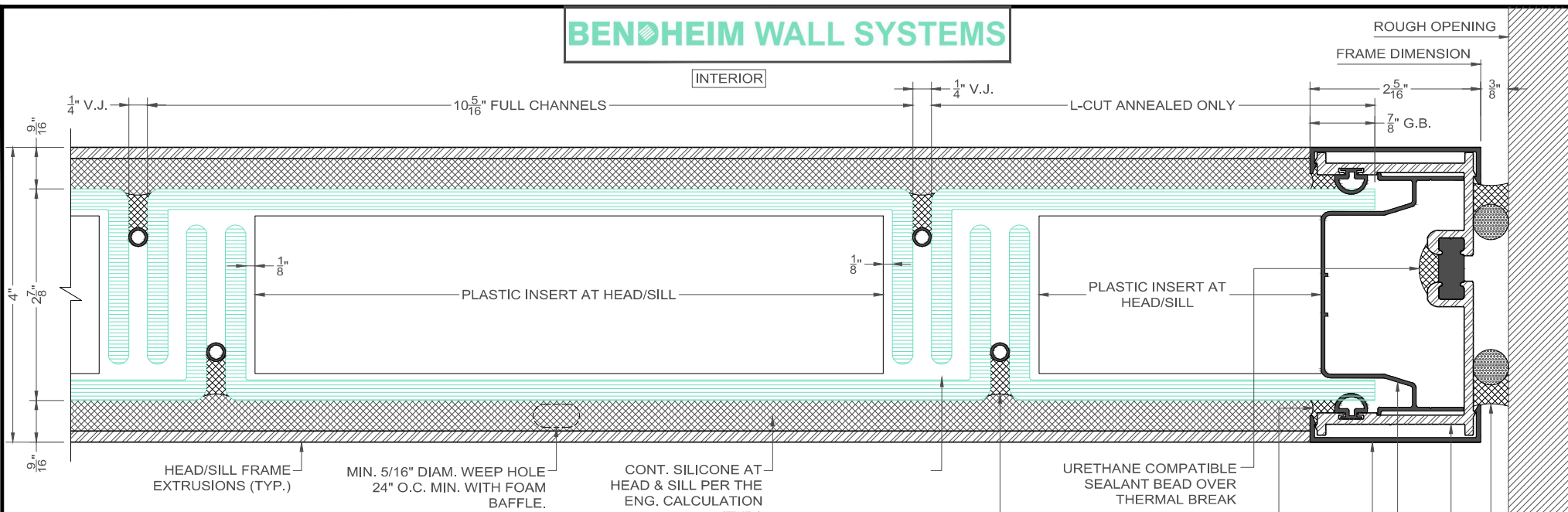
1 JAMB DETAIL WITH L-CUTS SD-3 SCALE: 6" = 1'-0"
