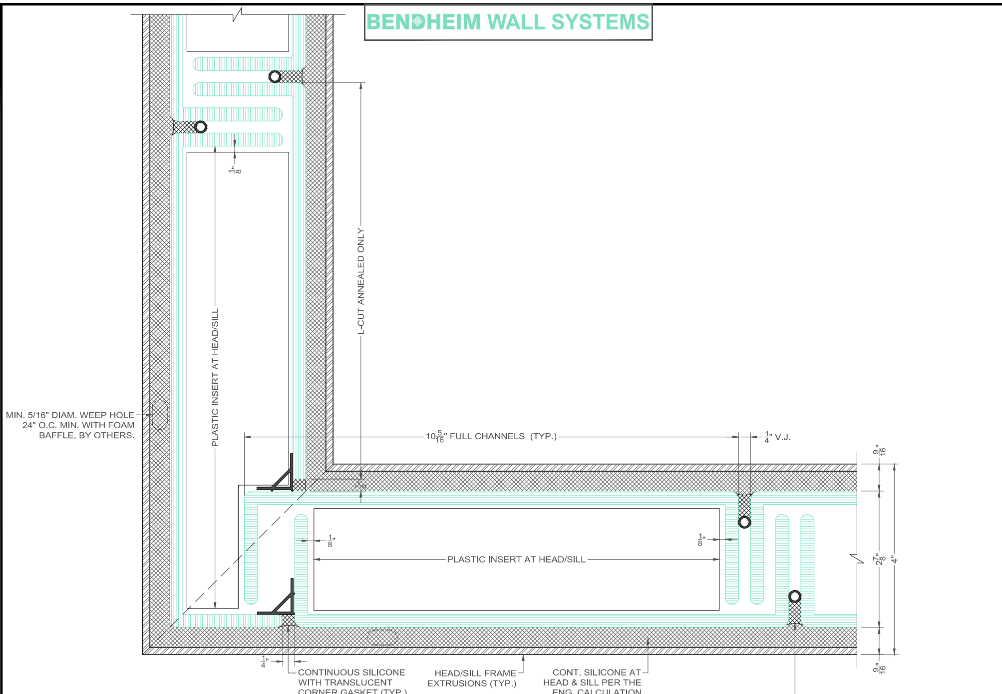
1 TYPICAL CORNER DETAIL SD-4 SCALE: 6" = 1'-0"
