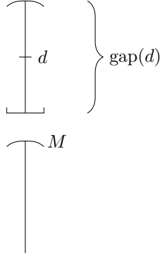
Figure 10.2: Extension of M \models \text{PA} by d realizing an unbounded strongly definable type
