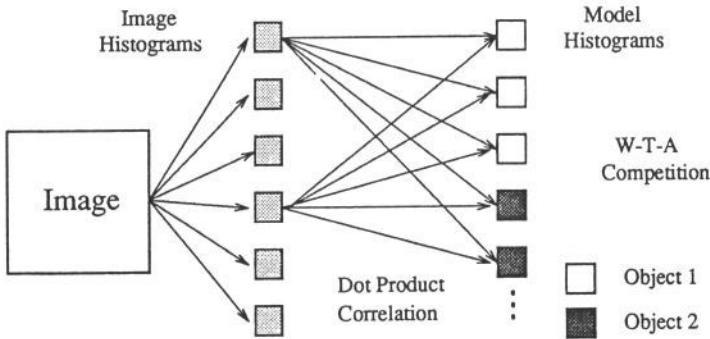
Fig 6: The Parallel Matching Strategy
