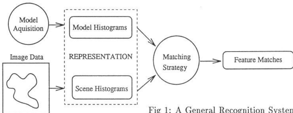
Fig 1: A General Recognition System
