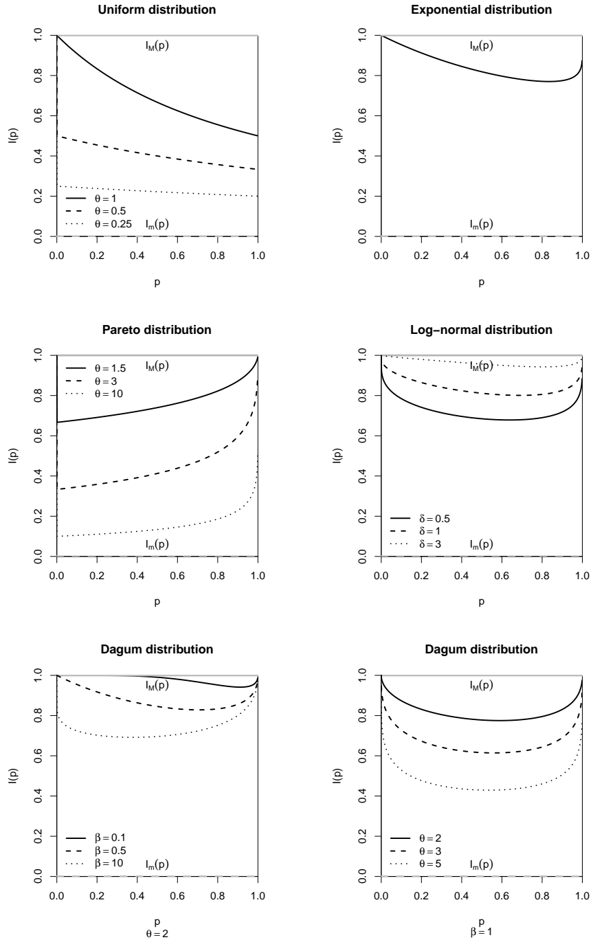
FIGURE 3: Graphs of different I(p) curves for the considered models
