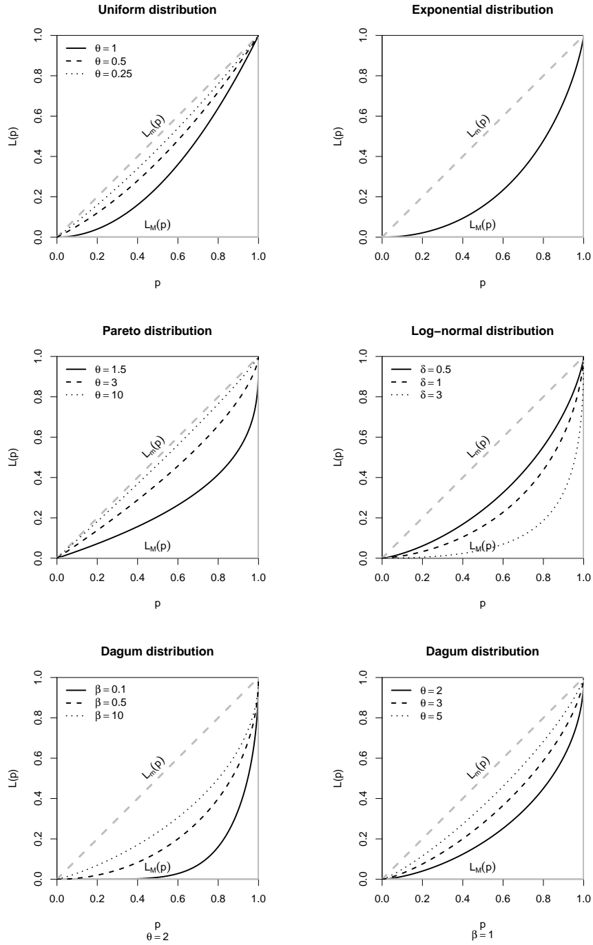
FIGURE 1: Graphs of different Lorenz curves for the considered models
