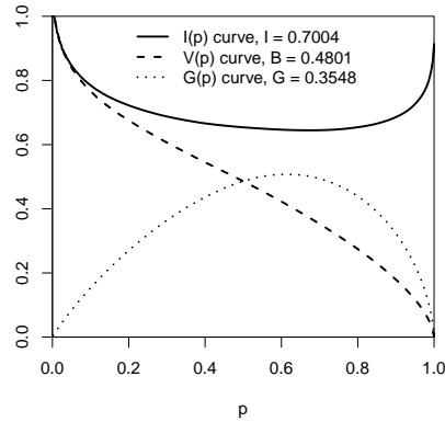
FIGURE 4: Unified representation of the inequality curves
