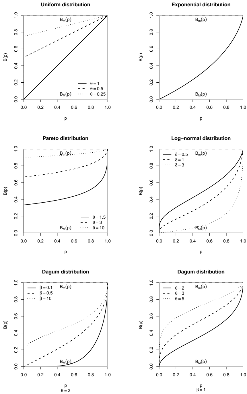
FIGURE 2: Graphs of different Bonferroni curves for the considered models
