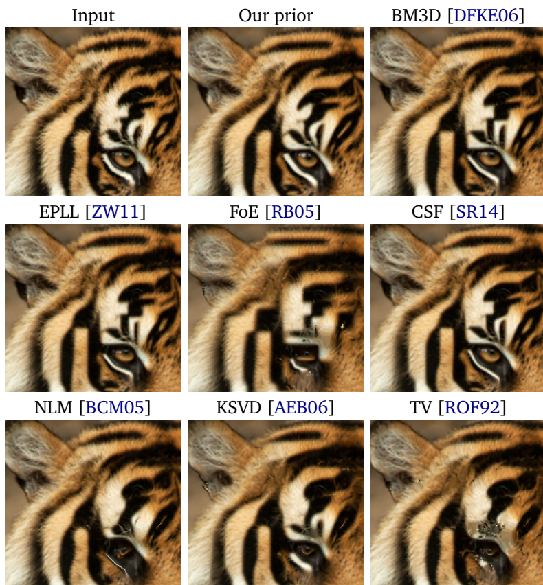
Figure 3.2: Visualization of image priors using the method by Shaham et al. [SM16]: Our deep mean-shift prior learns complex structures with different curvatures. Other priors prefer simpler structures like lines with small curvature or sharp corners.
