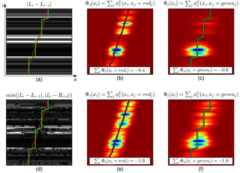
Figure 2.2: Visualization of the smoothness energy in the joint pixel-disparity space (pixels i on vertical axis, disparities d on horizontal axis). The top row shows the conventional approach, and the bottom row is our technique, where (a) is the conventional disparity discontinuity indicator, and (d) our proposed one. The red line in the left and middle column indicates the ground truth disparities, and the green line in the left and right column is a piecewise fronto-parallel disparity assignment. In the conventional approach, the piecewise fronto-parallel disparities incorrectly have a lower smoothness energy ( -0.6 in (c)) than the ground truth ( -0.4 in (b)). Our technique correctly leads to a lower energy for the ground truth ( -1.9 in (e)) compared to the fronto parallel disparities ( -1.8 in (f)).
