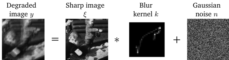
Figure 3.1: Our framework is built to restore degraded image y that is modeled as an unknown image \xi , blurred by convolution kernel k and corrupted with additive Gaussian noise n with variance \sigma_n^2 .
