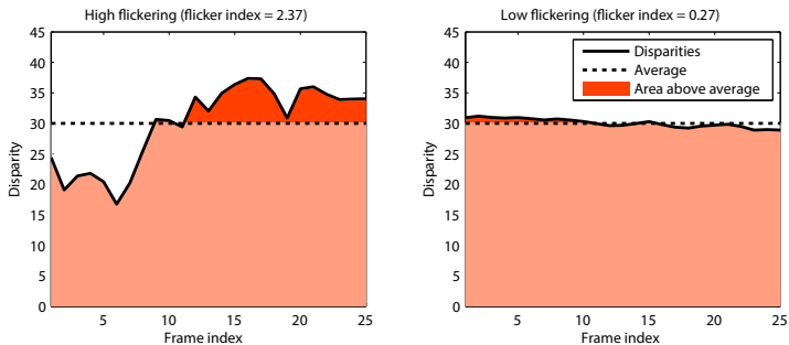
Figure 2.9: Visualization of the flicker index for tow disparity sequences. We compute the flicker index by taking the ratio of between the time-averaged disparities and the disparities above this average. This index is high in case of rapid changes of disparities in a time window (left), and is low for smooth transition of disparities (right).
