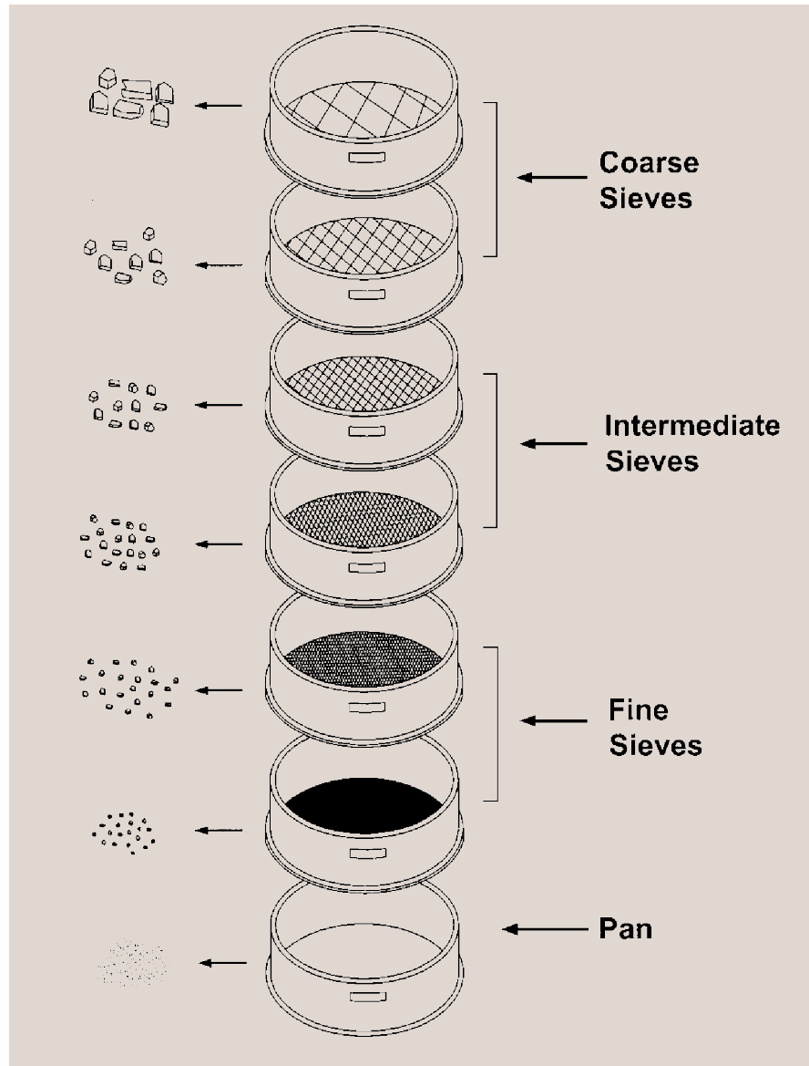
Figure 9: Stack of sieves used for testing the gradation of aggregate.
