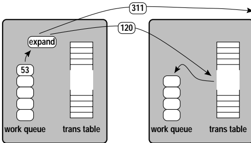
Figure 2: Transposition-driven scheduling.
