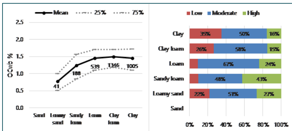
Figure 1. Mid North topsoil average SOC %, number of samples, upper (75%) and lower (25%) bands (left) and proportion of texture samples in the high, moderate and low SOC range (right) for texture.
