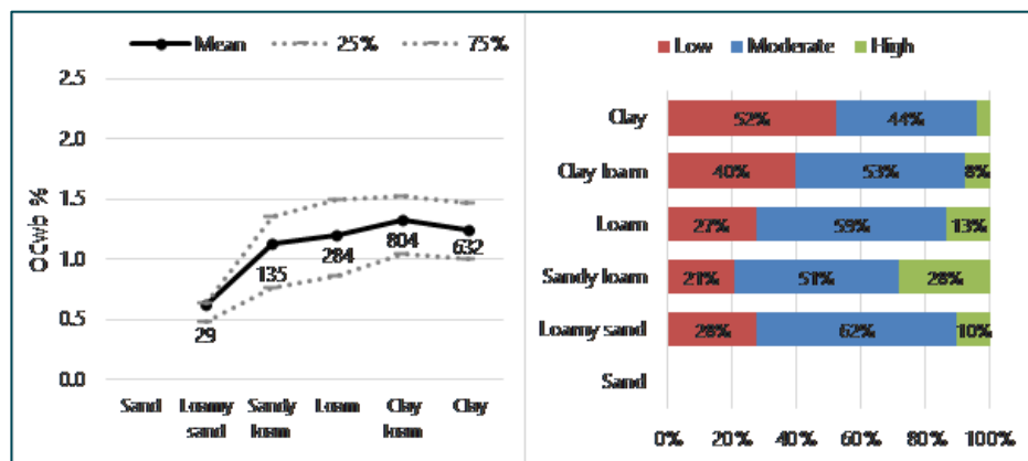
Figure 1. Upper North topsoil average SOC %, number of samples, upper (75%) and lower (25%) bands (left) and proportion of texture samples in the high, moderate and low SOC range (right) for texture.
