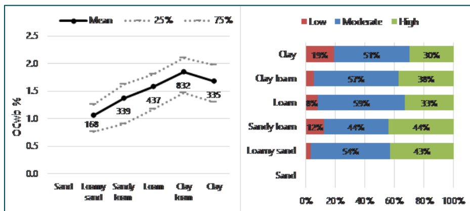
Figure 1. Yorke Peninsula topsoil average SOC %, number of samples, upper (75%) and lower (25%) bands (left) and proportion of texture samples in the high, moderate and low SOC range (right) for texture.
