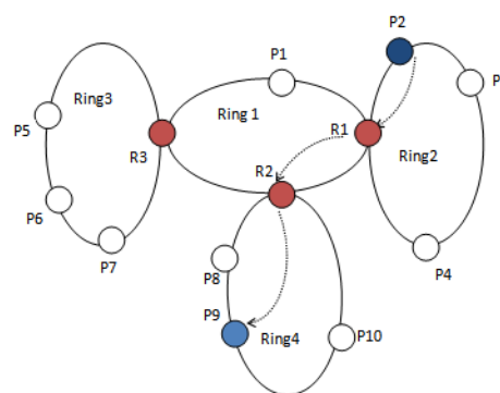
Figure 2: example of lookup and download in HPM
