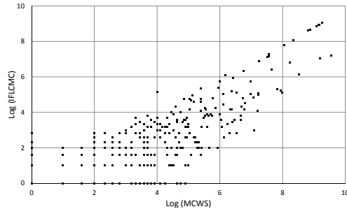
Fig. 7. Analyzing hierarchical height and featureless metaclasses
