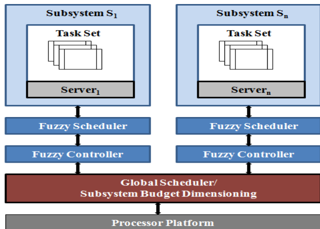
Figure 1: AHS-RT Architecture
