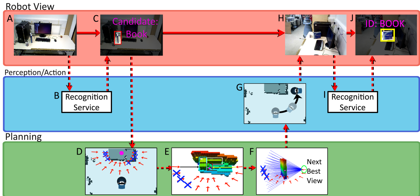
Figure 3: The next best view planning process step-by-step: A: Receive initial view. B: Recognition service processes point cloud. C: Candidate object and pose identified. D: Collision detection around object location. E: Environmental analysis for occlusions (candidate object in pink, occlusions in white and blue). F: Model analysis with remaining rays. G: Move to best view pose. H: New point cloud sent to recognition service and object recognised. I: Point cloud from second view is sent to recognition service. J: Visualisation of recognition service correctly and fully recognising the target object.
