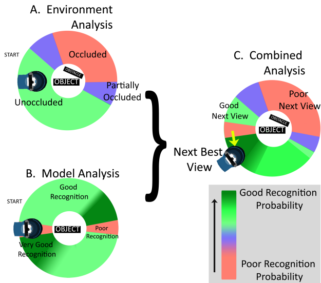
Figure 1: Next best view planning: Conceptual overview. The approach has two steps: (A) an environmental analysis and (B) a model analysis. The analysis of the environment reasons about the visibility of an object and is carried out based on a set of navigable poses. Poses in suitable areas are then carried on into the model analysis (B), in which the visibility of object features is evaluated. Conceptually, the resulting areas from (A) and (B) are combined to find the next best view (C).
