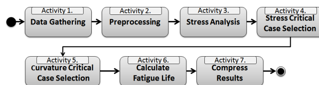
Figure 1. Risers Fatigue Analysis Workflow.
