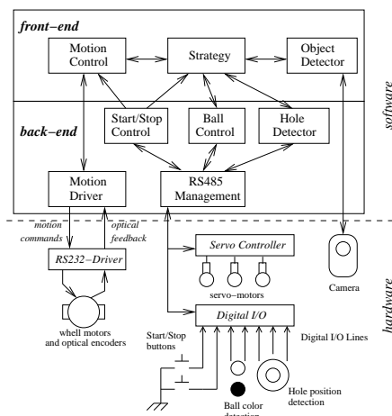
Fig. 3. Hardware/Software Architecture
