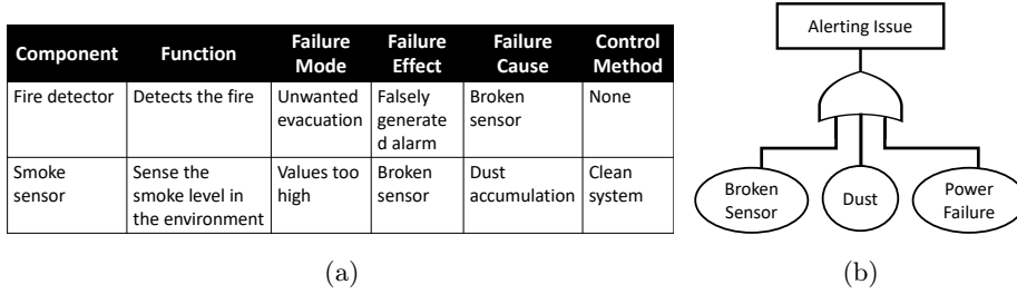
Fig. 1: Example of FMEA (a) and FTA (b)
