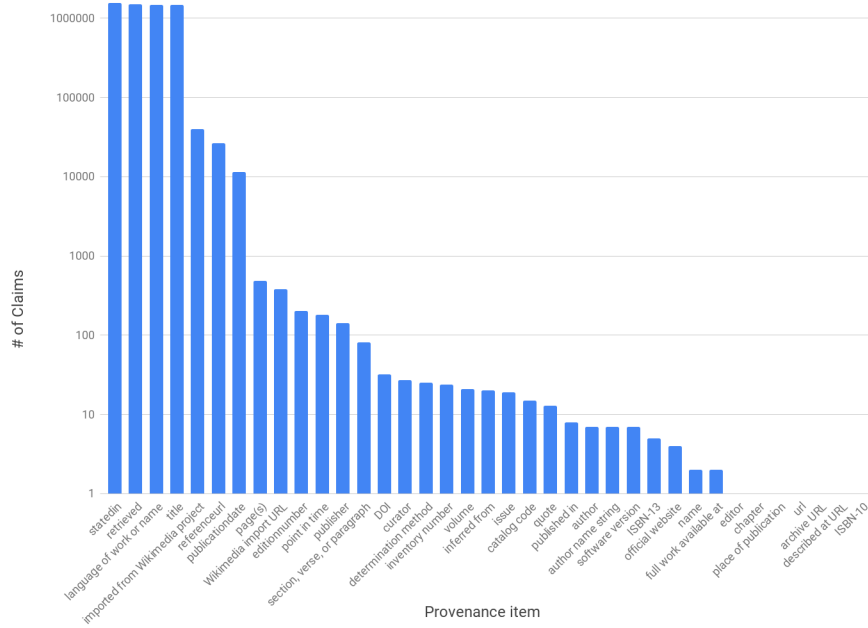
Fig. 2. Usage frequency of each provenance item in Wikidata.
