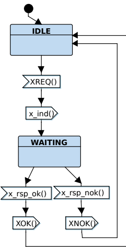
Fig. 7. Protocol Machine for the Responder
