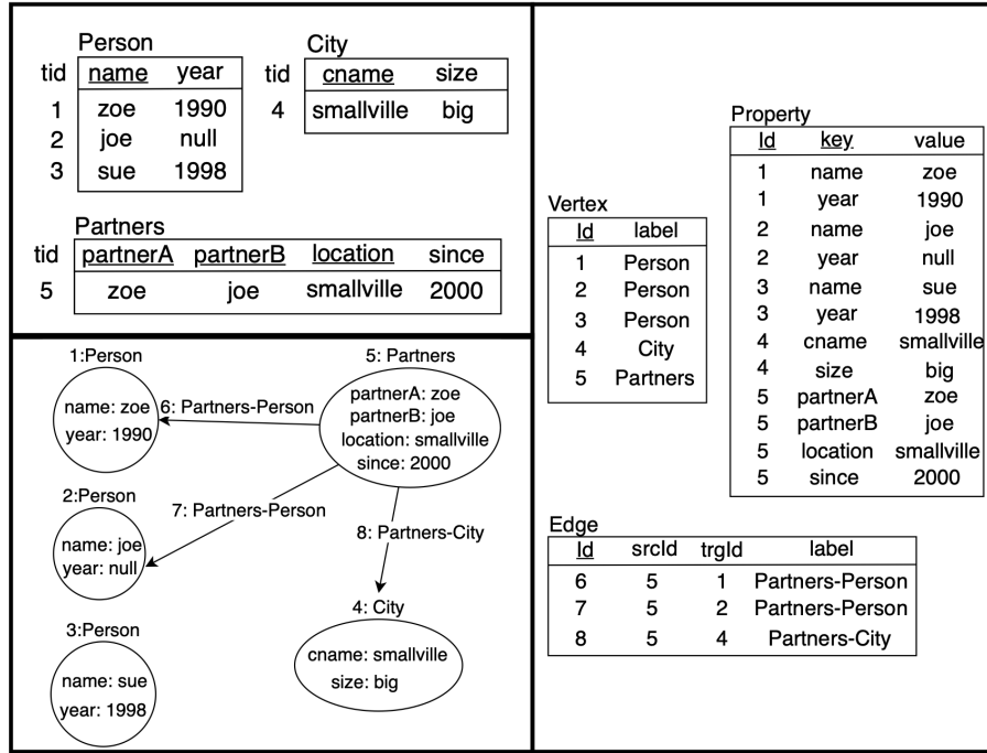
Fig. 1. (top left) An RDB (\mathbf{S}, \mathbf{I}) , where primary key attributes are underlined, partnerA and partnerB of Partners are foreign keys to name of Person , and location of Partners is a foreign key to cname of City . (bottom left) The property graph \text{R2PG-DM}(\mathbf{S}, \mathbf{I}) and (right) its representation with predicates Vertex , Edge , and Property .
