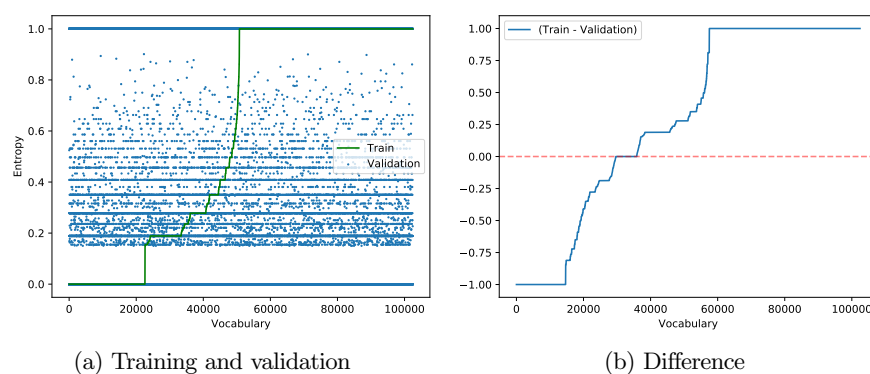
Fig. 2. Vocabulary relevance for training and validation
