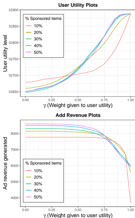
Figure 2: User utility and ad revenue curves estimated for real data from an online grocery retailer
