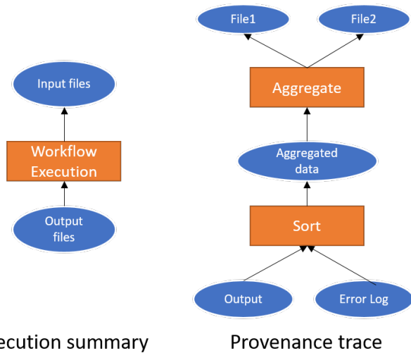
Figure 2: An example of a simple provenance summary. The execution of a workflow on the right is summarized as a single activity on the left. Arrows represent usage/generation dependencies.
