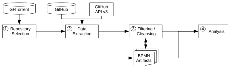
Fig. 1. Schematic illustration of the mining pipeline.
