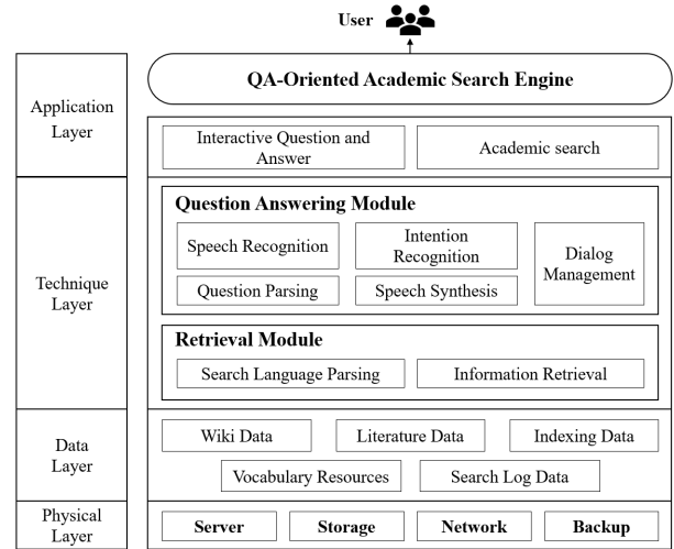
Figure 3: System Framework.
