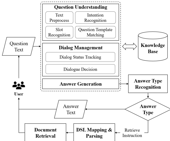
Figure 2: Dialog System Framework.
