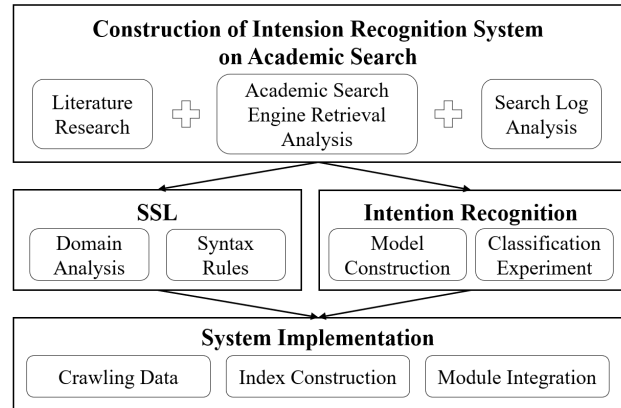
Figure 1: Research Framework.
