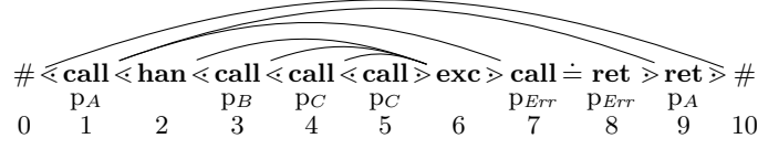
Fig. 2. The example string as an OP word. Chains are highlighted by arrows joining their contexts; structural labels are in bold, and other atomic propositions are shown below them. p_i means a call or a ret is related to procedure p_i . First, procedure p_A is called (pos. 1), and it installs an exception handler in pos. 2. Then, three nested procedures are called, and the innermost one ( p_C ) throws an exception, which is caught by the handler. Function p_{Err} is called and, finally, p_A returns.
