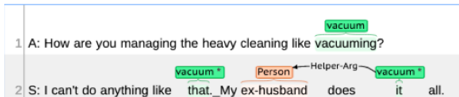
Figure 2: Example dialogue annotated for semantic frames.
