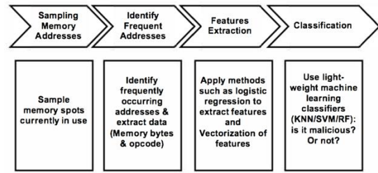
Figure 3: Malware/anomaly Detection with Light-weight Machine Learning Methods
