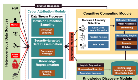
Figure 1: Comprehensive Architecture of Secure Intelligent Autonomous Systems with Cyber Attribution
