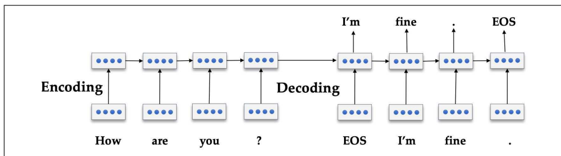
Fig. 1. A sequence to sequence model for neural response generation in dialog. [8]
