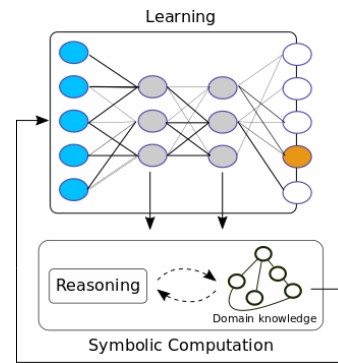
Figure 6: Hidden layer integration: reasoning is applied upon hidden layers of neural networks.
