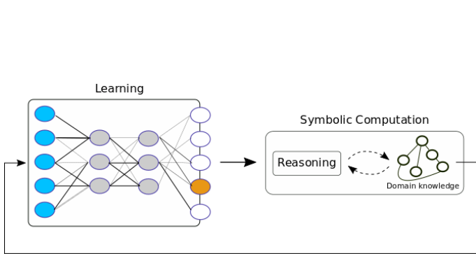
Figure 5: Boundary integration: reasoning is applied upon boundary layers of neural networks.
