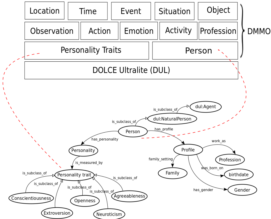
Figure 8: The Digital Mental Model Ontology (DMMO) is a network of ontology patterns representing different aspects of the mental model of a user. The patterns are interlinked through general classes in the upper ontology DOLCE UltraLite. For instance, the two patterns Person and Personality Traits are linked through the class person subsumed by the shared class dul:NaturalPerson.
