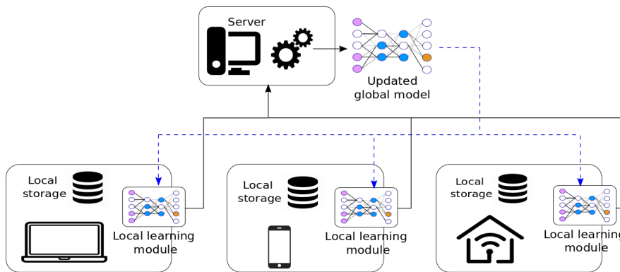
Figure 7: An overview of federated learning.
