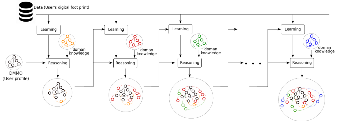
Figure 4: Neural-symbolic integration approach to build an ontological digital mental model of a user (DMMO ontology) based on her digital footprints.
