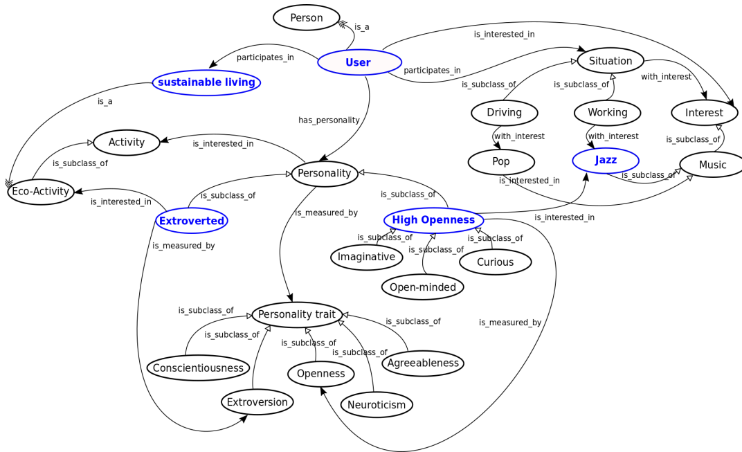
Figure 11: Populated DMMO based on the best possible explanations inferred from data.
