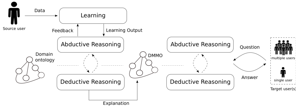
Figure 9: A high level view on building and using DMMO based on interactions between learning and reasoning modules.
