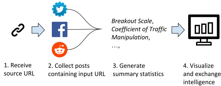
Fig. 1: Information Tracer Architecture. The input to the system is a valid URL. Upon receiving the URL, our system automatically collects posts containing this URL from designated social networking platforms, generates aggregated statistics, and finally presents results on a web interface.
