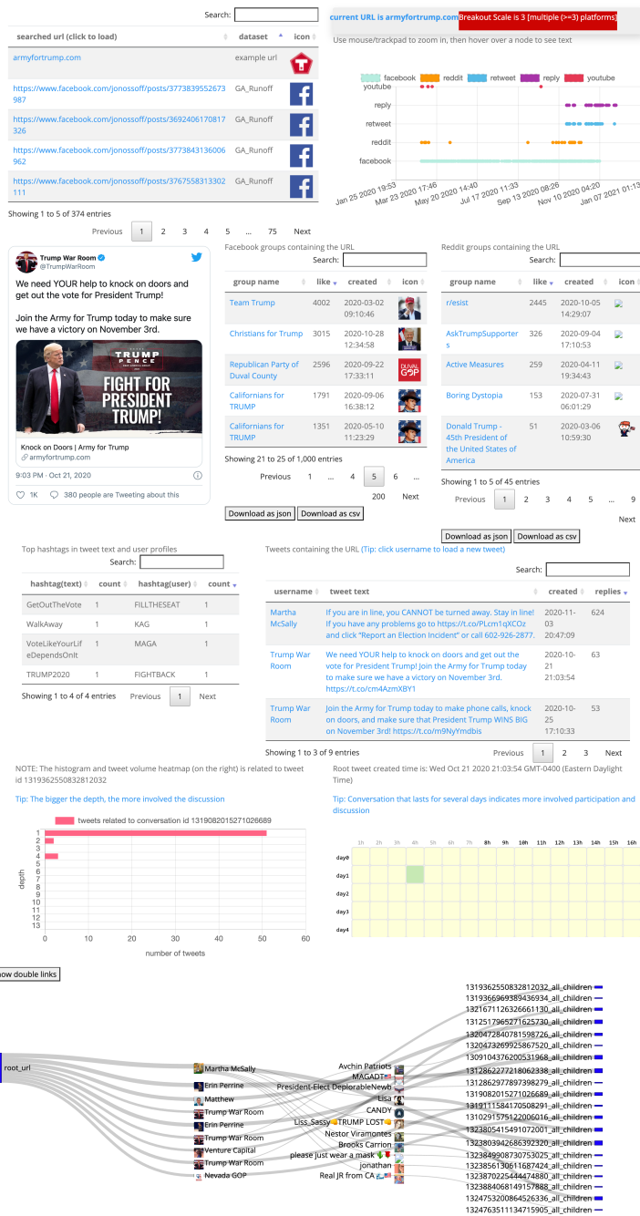
Fig. 2: Information Tracer User Interface. This detail page visualizes the spread pattern of URL armyfortrump.com . To understand when people share the website, one can examine the scatter plot (first row). To understand who shares, one can inspect top Facebook groups, top Reddit groups, and top original tweets (second and third row). Finally, to understand how conversation unfolds, one can check the retweet and reply networks (bottom row).
