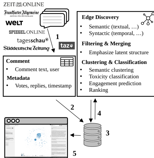
Figure 1: The ComEx system transforms comments into a graph structure and allows their exploration through a web interface.
