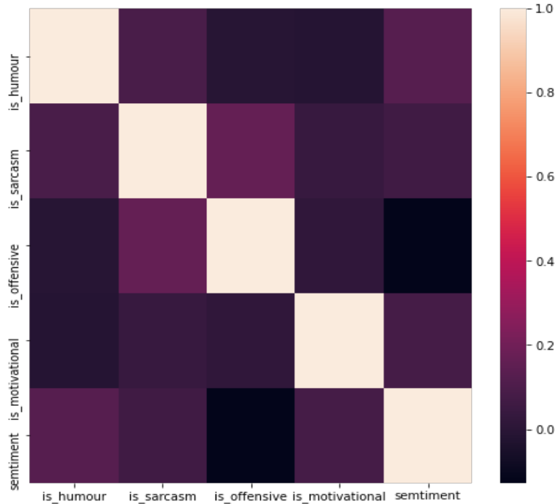
Figure 2: Correlation among labels: sentiment (task A) has positive correlation with is_humour (task B) but negative relation with is_offensive (task B)
