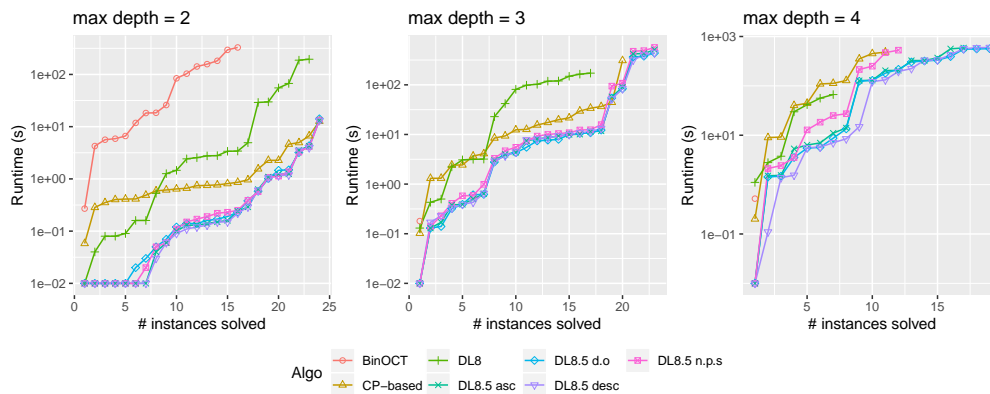
Figure 1: Cumulative number of instances solved over time
