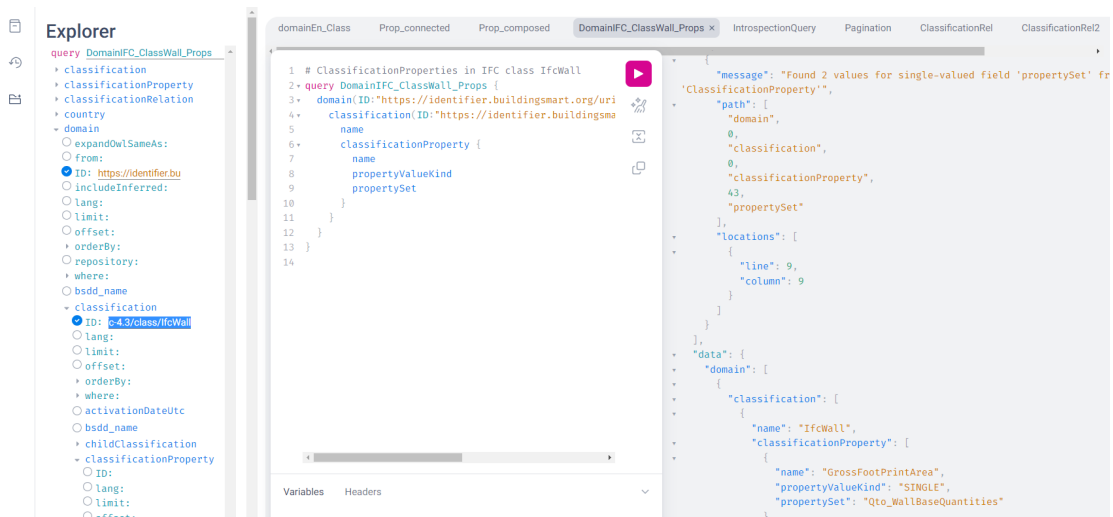
Figure 3: GraphQL Querying of Refactoring bSDD Endpoint
