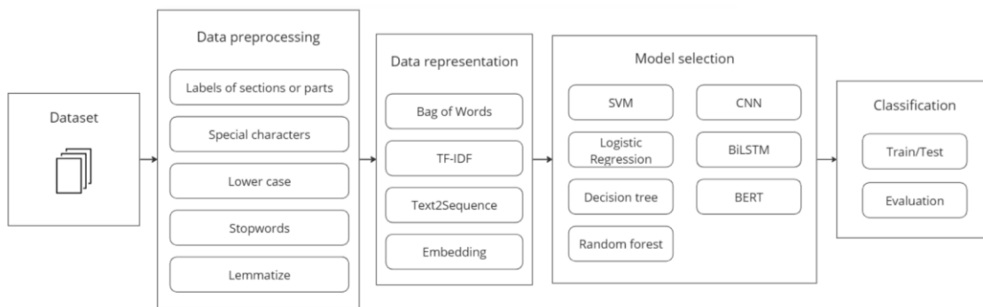
Figure 1: Methodology for hate speech detection in lyrics using traditional machine learning algorithms and transformer models.
