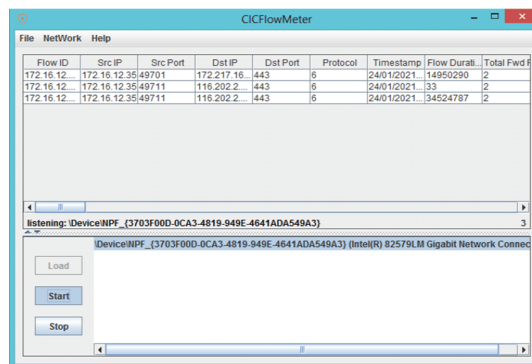
Figure 1: Example of the CICFlowmeter’s GUI
