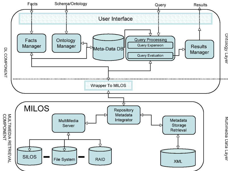
Fig. 1. DL-MEDIA architecture.
